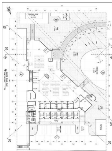
Gambar 1 Layout awal lantai 1
